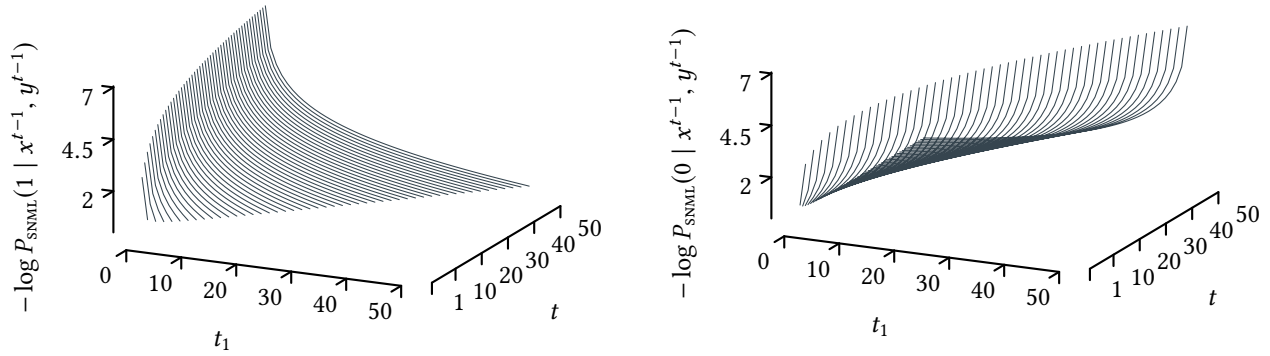
Figure 1: SNML predictions using the past of x^n , and that of y^n . For time steps t = 1, 2, \dots, 50 , and number of ones in the past t_1 = 1, 2, \dots, 50 such that t_1 < t , we plot the code length using the SNML prediction strategy for (left) x_t = 1 , and (right) x_t = 0 .
